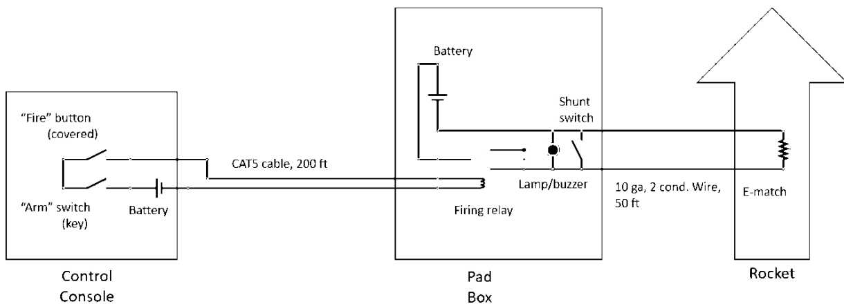
Figure 2, An improved high current fire control system.
